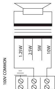
Circuit Diagram
