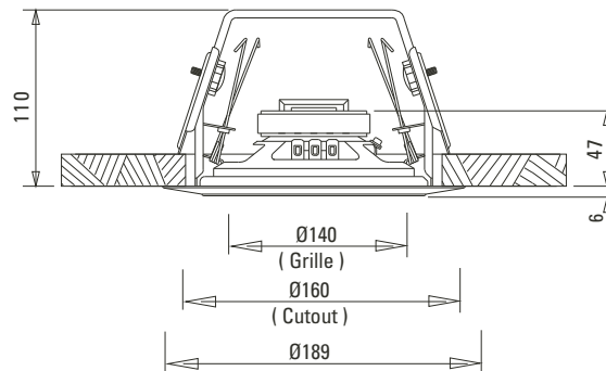
Side view (unit: mm)
