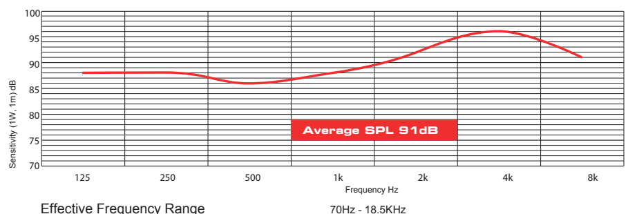
Frequency response
