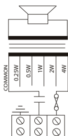
Circuit Diagram
