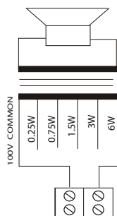
Circuit Diagram
