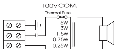
Circuit Diagram
