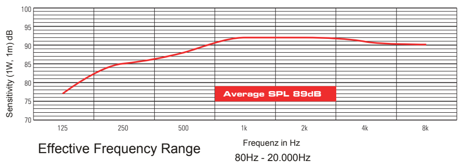
Frequency response
